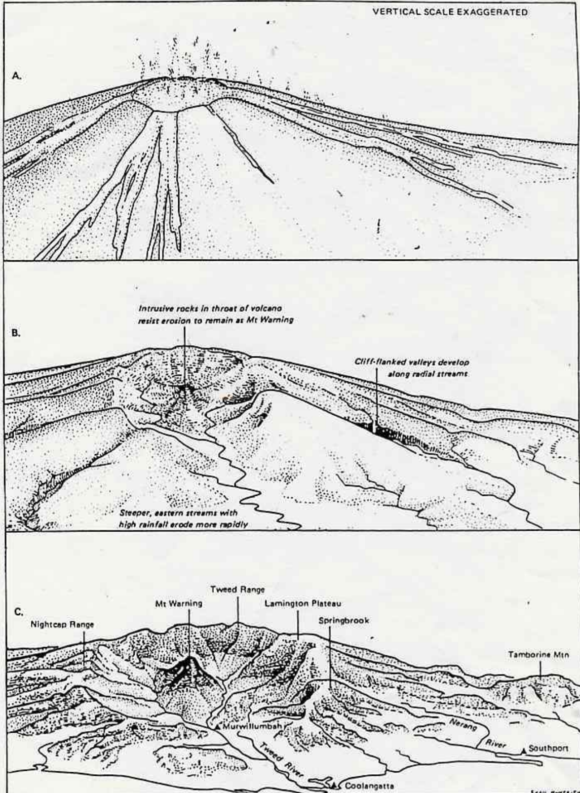
Progressive erosion of the Tweed Volcano.
